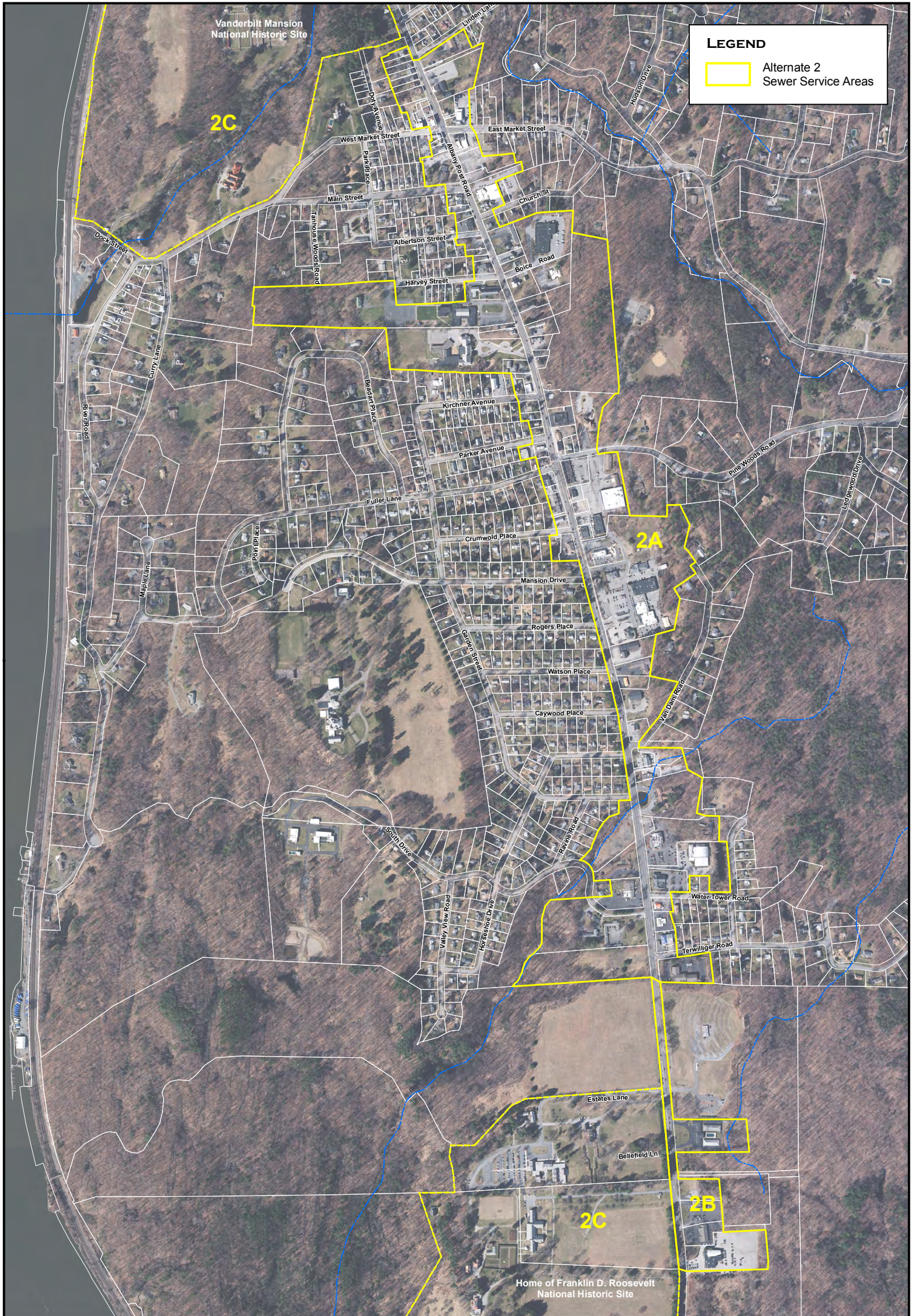
FIGURE 2 REVITALIZING HYDE PARK'S TOWN CENTER ALTERNATE 2 - ROUTE 9 COMMERCIAL SEWER DISTRICT DUTCHESS COUNTY, NEW YORK
